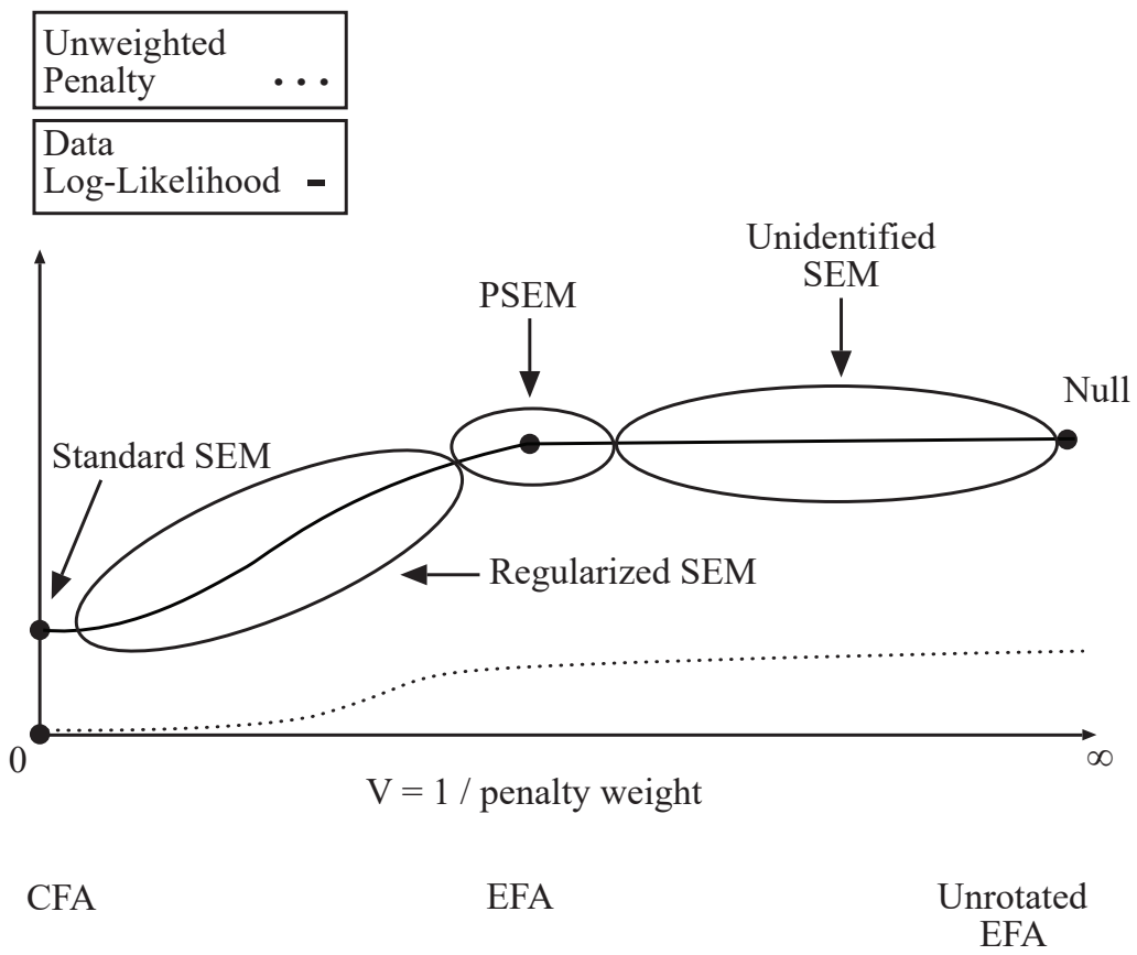
Figure 2: Penalty weight effect on models
