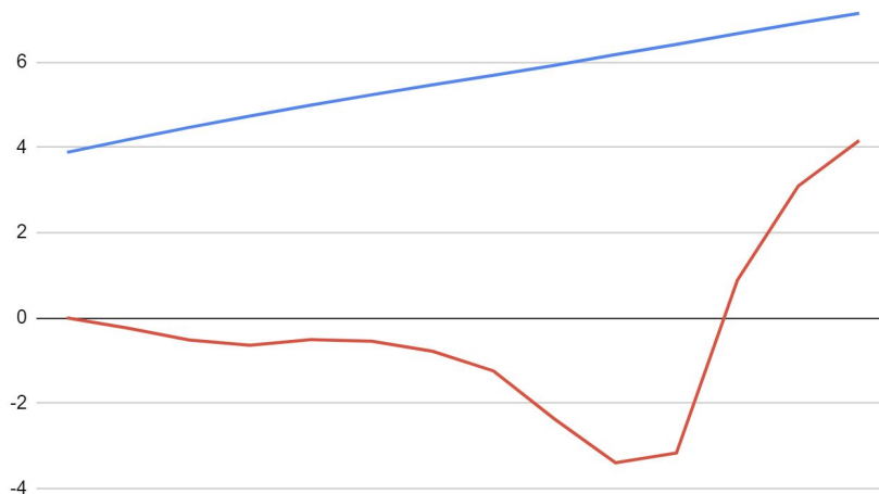
Figure 3: The two predictor curves for the height model
