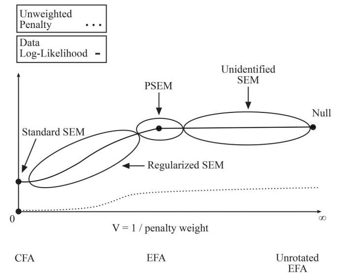
Figure 2. Penalty weight effect on models.
